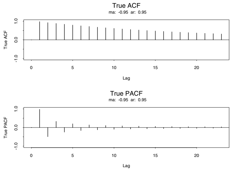
Figure 11: True ACF and PACF for ARMA(1,1) model with \phi_1 = 0.95, \theta_1 = -0.95
